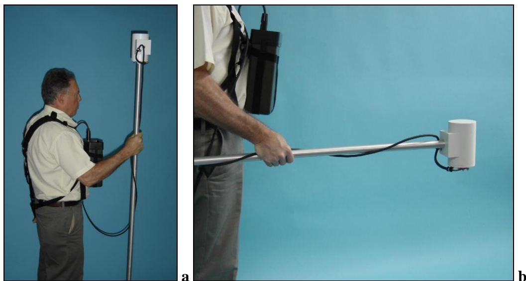
Figure 7. Assembled magnetometer
