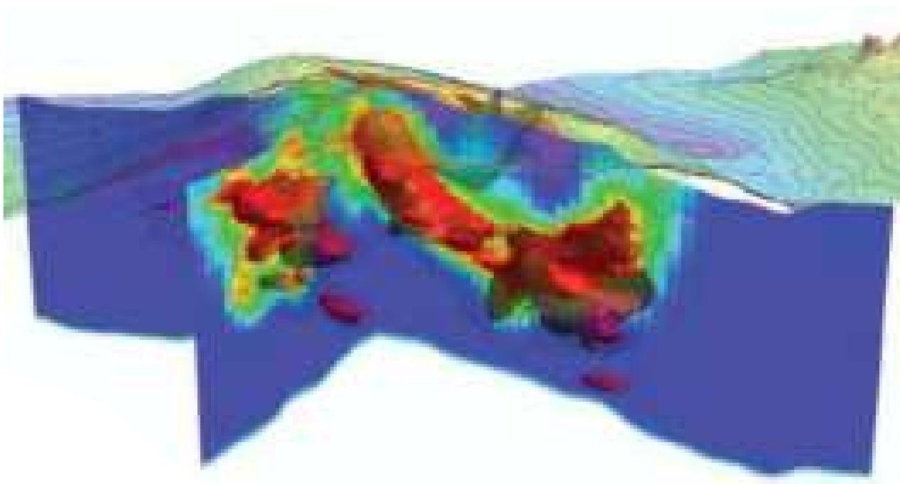
3D conductivity iso-surface showing buried geological targets.
