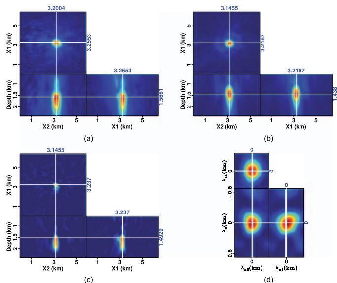
Figure 10. Zero-lag image volumes (a) PP, (b) SS, and (c) PS using the inverted velocity model and data of the moderate event shown in Figure 3d–f and (d) shows a slice through the extended PS image volume extracted at the maximum location of the zero-lag image (from Witten and Shragge, 2017b).
