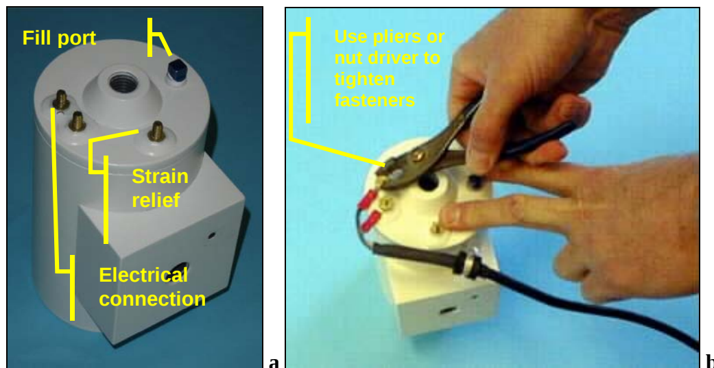
Figure 3. Sensor preparation.
