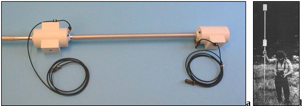
Figure 14. Completed gradiometer staff.
