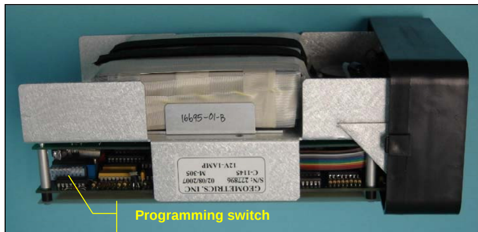
Figure 22. Location of console's internal programming switch.
