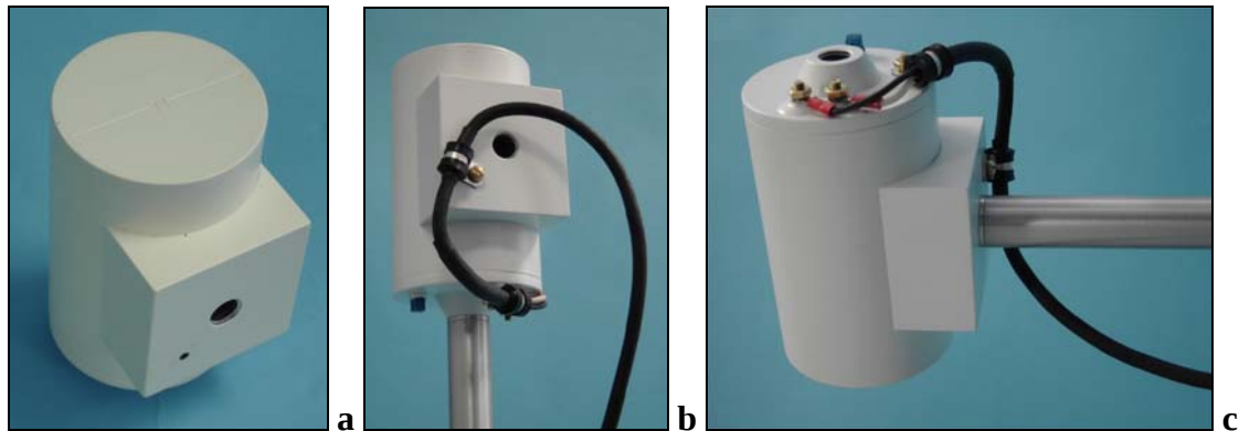
Figure 17. Alternate orientation for G-856AX sensor mount.
