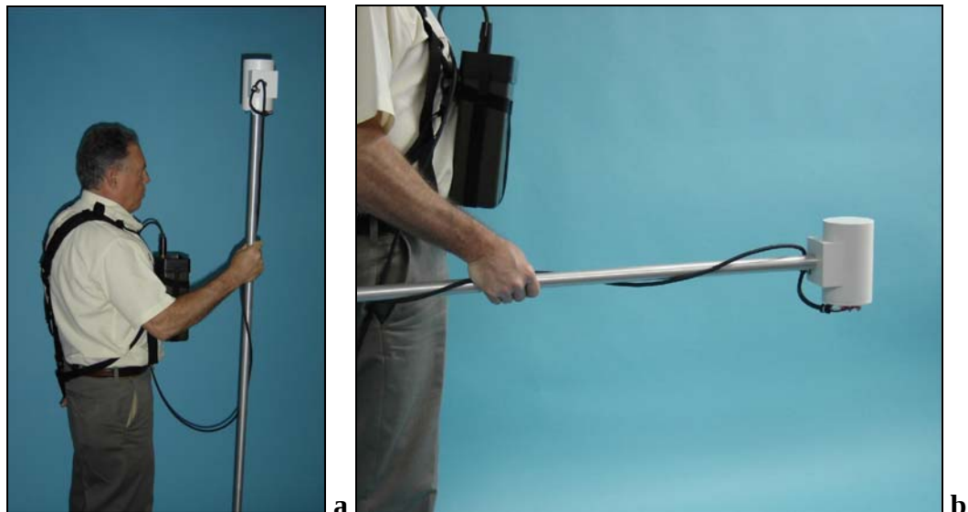
Figure 7. Assembled magnetometer.
