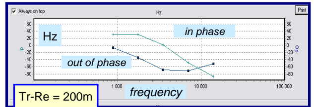
PROMIS FREQUENCY EM SOUNDING with 50m, 100m, 200m Tr-Re spacings, Orléans Loire River site, France
