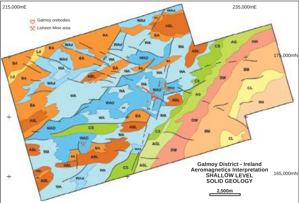
Figure 10.24: Shallow solid geology interpretation.
