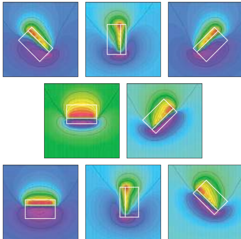
Figure 2.11: Pb block model (depth 100 m) dipping at 45^\circ for a range of strike directions. Calculated at Earth's field inclination of -50^\circ . Note in particular that when the dips are to the south, the asymmetry of the anomaly gives the impression of northerly dip. The equivalent northern hemisphere models can be observed by rotating the diagram 180^\circ .
