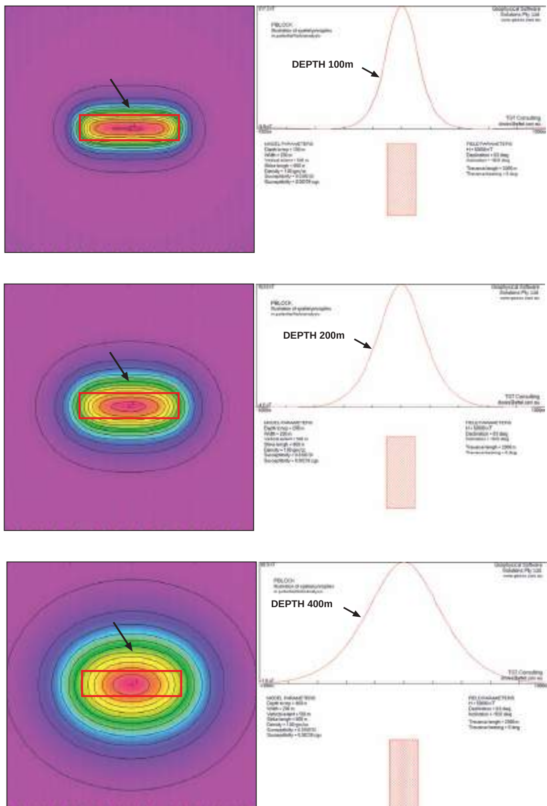
Figure 2.5: Pb block model at Earth's field inclination of 90° (polar regions) showing the link between body location and maximum gradient position (arrowed) for varying depths. The profiles cross the centre of the body.
