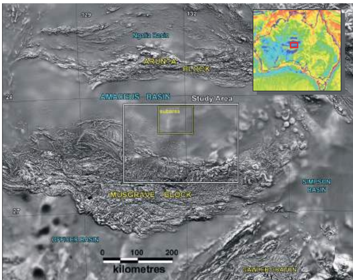
Figure 13.1: Location diagram, Amadeus Basin study area. Underlay is the TMI aeromagnetic grid of Australia. Inset shows the location in the continental context; underlay is the Bouguer gravity grid of Australia. Note the extreme gravity variations in and near the study area. Data courtesy Geoscience Australia.
