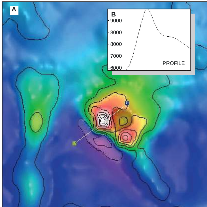
Figure 3.31: Self-demagnetisation effects at Trough Tank (Osborne) (adapted from Gidley 1988).
