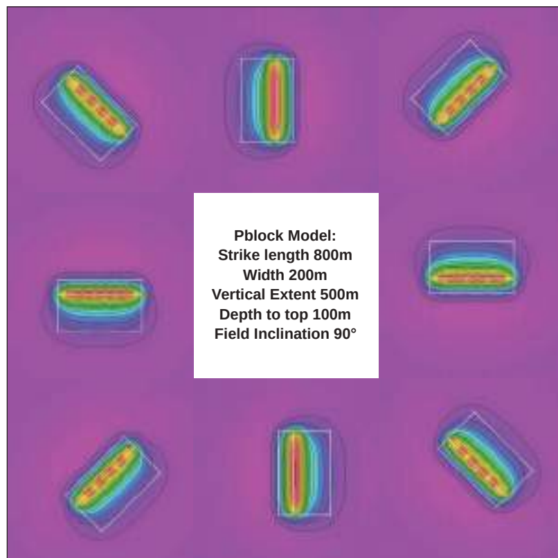
Figure 2.12: Pb block model (depth 100 m) dipping at 45^\circ for a range of strike directions. Calculated at Earth's field inclination of 90^\circ . Because the Earth's magnetising field is vertical in this example, the anomaly asymmetry closely reflects the geometry of the model body.
