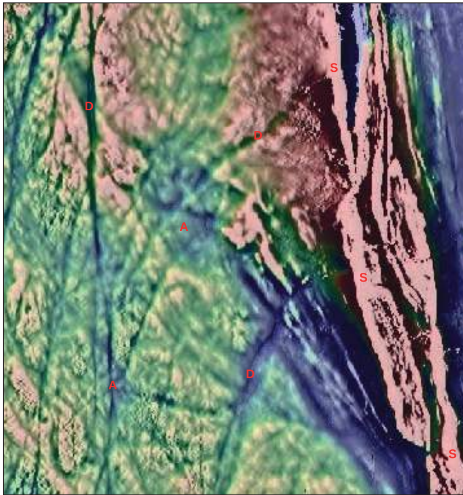
Figure 3.15: Magnetic alteration effects in the Goongarrie district, WA. Data courtesy UTS-Geophysics. S = indicates zones of serpentinitisation, D = magnetite destruction/haematite development in fault zones, A = alteration/ magnetite destruction zone at junction of faults and intrusive contact. The image is 15 km E-W.
