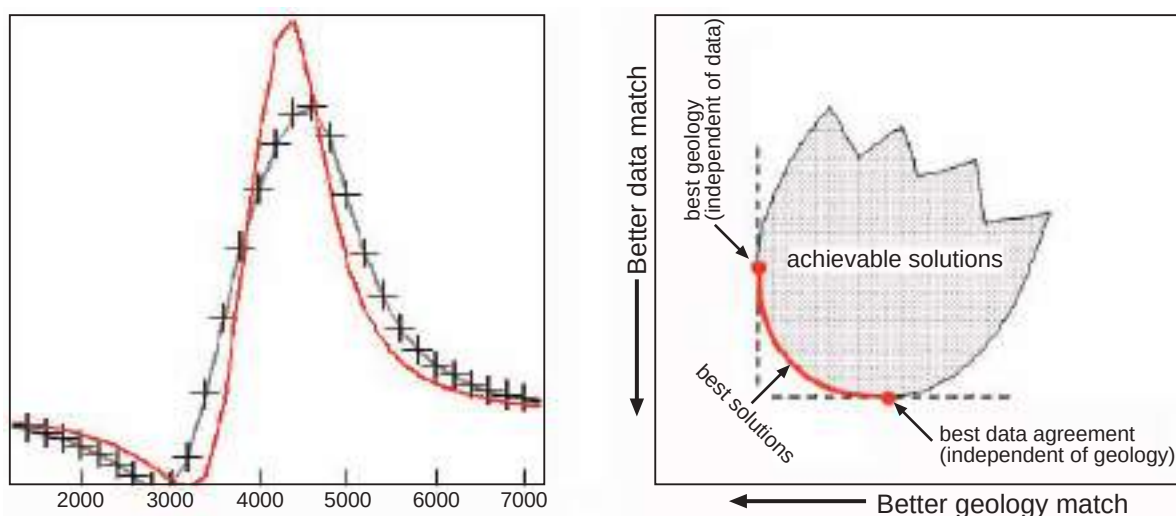
Figure 8.3: Illustration of inversion principles. At each iteration, parameter adjustments are made based on the mismatch between measured (crosses) and model data (red line). This proceeds until the sum of the squares of the differences reaches an acceptable minimum. The achievable solutions field in the right-hand graphic represents numerically acceptable minima in the sum of the squares of the differences. The 'best' solutions are where there is a balance between the closeness of the data match and adherence to geological constraints. Figure from Oldenburg and Pratt (2007).
