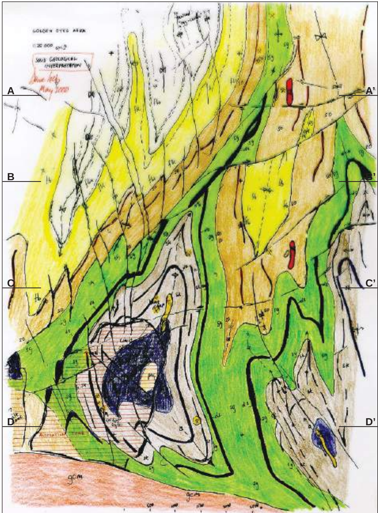
Figure 12.22: Working (draft) solid geology layer, showing cross-section locations. See Figure 12.20 for legend.
