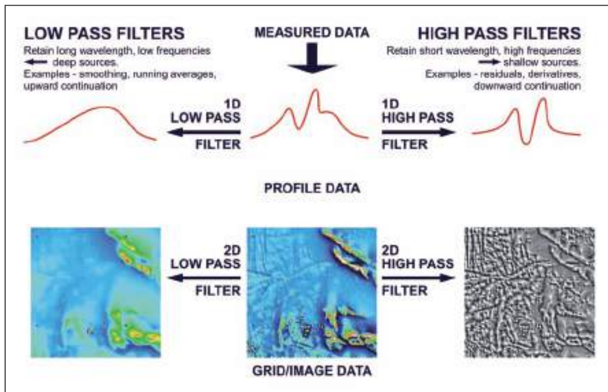
Figure 5.16: Summary of the mechanics of filtering.
