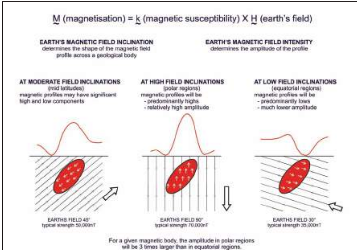
Figure 2.3: Illustration of rock magnetisation by magnetic induction.
