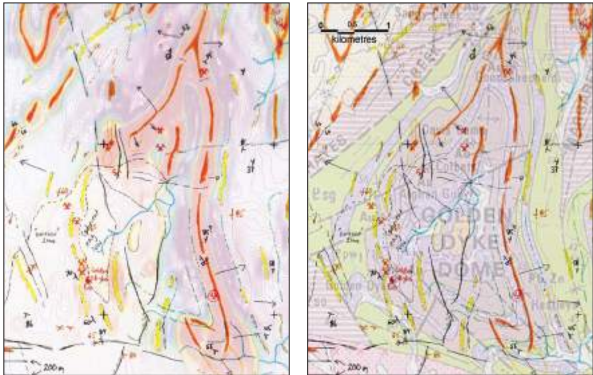
Figure 12.16a: Golden Dyke Dome – aeromagnetic observations on RTP 1st VD (left) and outcrop mapping (right). Refer to Figures 12.8, 12.12 and 12.14 for originals.
