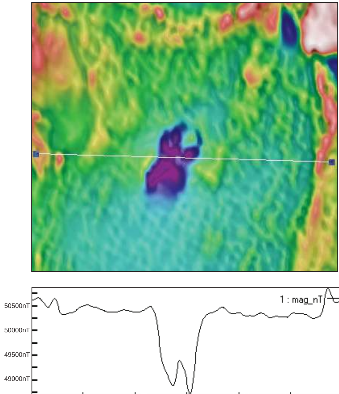
Figure 3.18: Biotite-magnetite alteration anomaly associated with the Mt Leyshon hydrothermal breccia pipe (Sexton et al. 1995). Note that in this case the magnetic response is anomalously negative indicating (chemical) remanent magnetisation. The profile is ~6 km long. Data courtesy Fugro Airborne Surveys.
