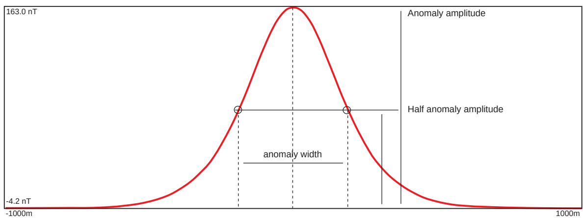
Figure 2.9: Graphical construction of ' \times 1/2 ', the width of the anomaly at half maximum amplitude.
