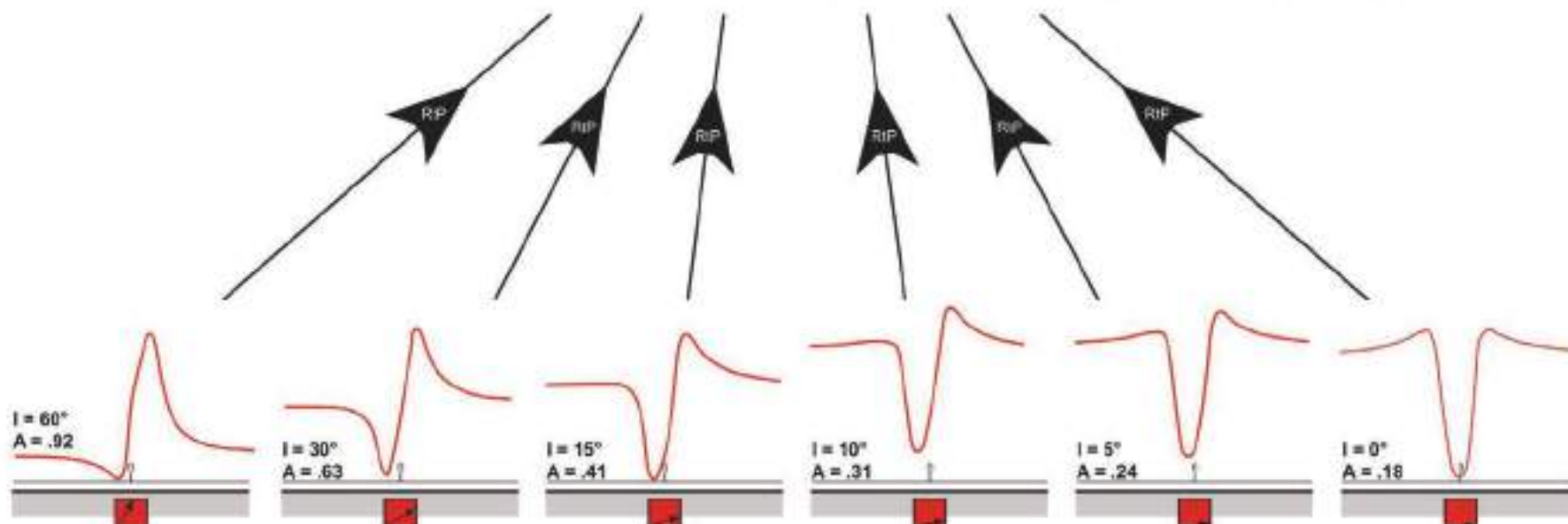
Figure 5.9: Illustration of the RTP process.
