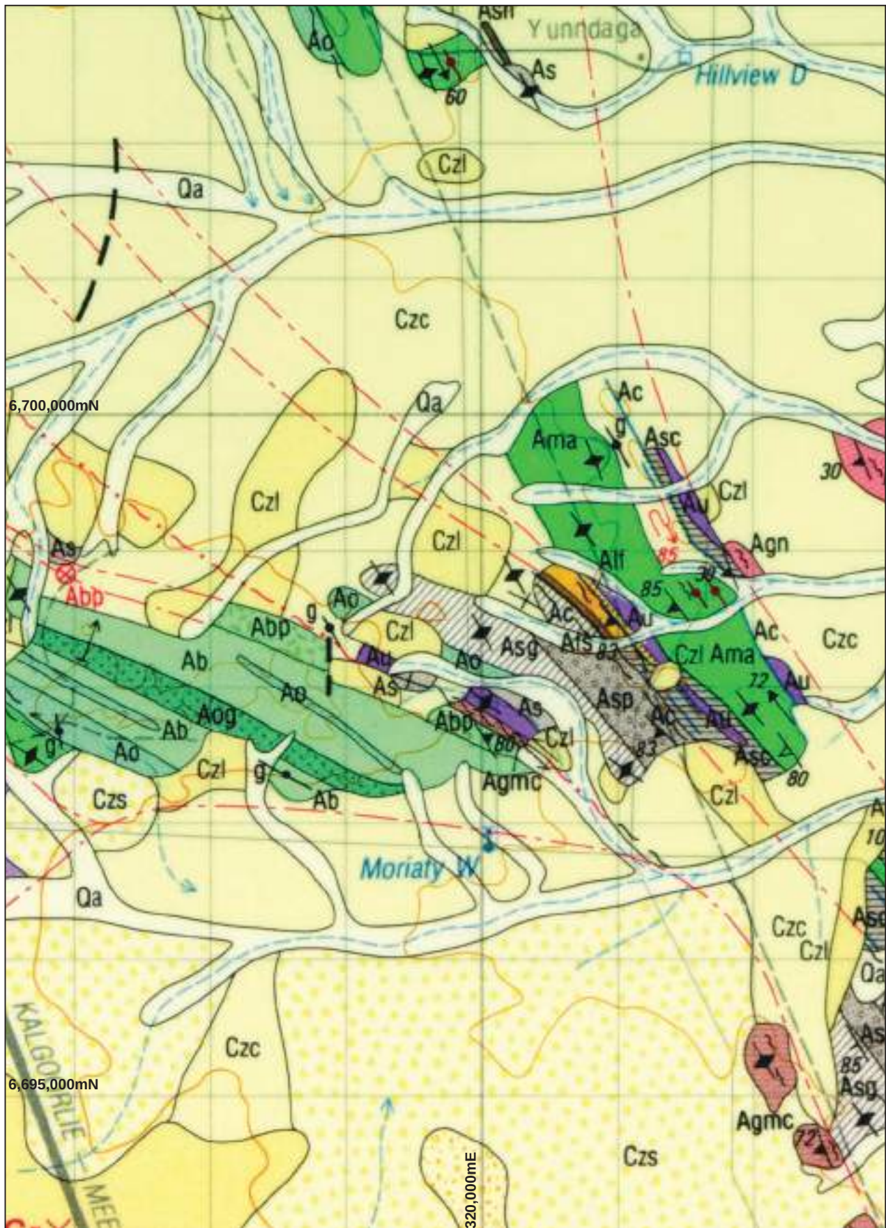
Figure 11.22: Moriarty Well area 1:25 000 scale study: Geological Survey of WA outcrop geology (part 'Menzies' 1:100 000 sheet, refer to Fig. 11.4b for legend). Grid is 1 km.
