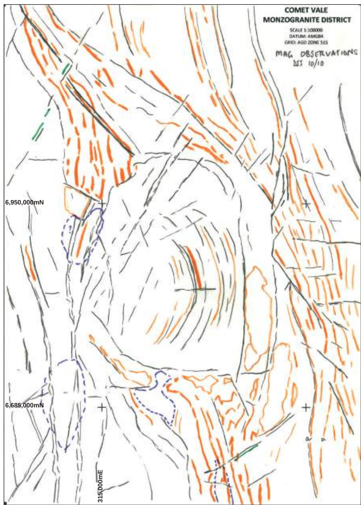
Figure 11.18: Observations layer (legend follows Figure 11.8).
