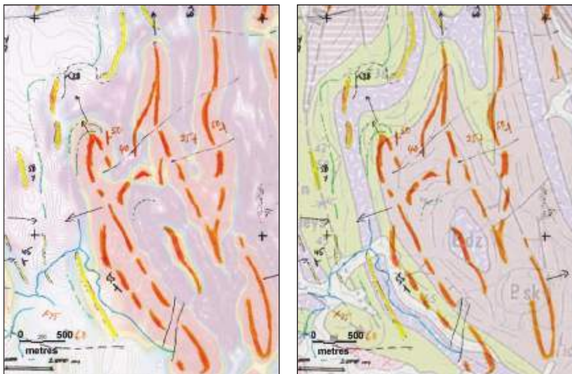
Figure 12.16b: South East Dome – aeromagnetic observations on RTP 1st VD (left) and outcrop mapping (right).
